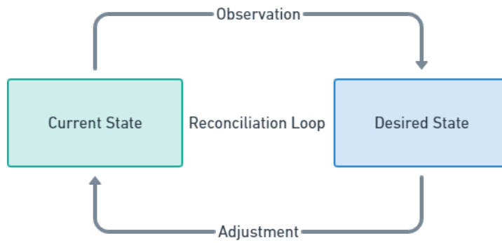
Figure C.1: The Kubernetes reconciliation loop. It can be compared to a basic feedback control system that reacts based on system output with a controller [23].
