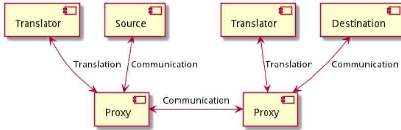
Figure 17: Networking with a Proxy
