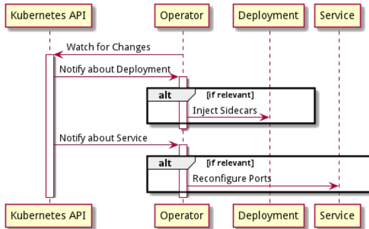
Figure 13: Automated Enhancement of a Deployment and a Service. If the Operator decides that an object is relevant (see Figure 12), the object is enhanced depending on its type.
